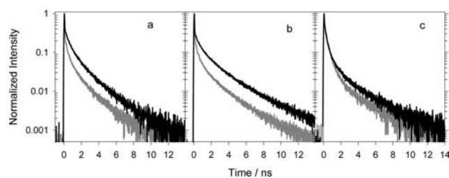
Figure 3. Fluorescence decays of DNA in water (gray) and in phosphate buffer (black) recorded at 305 nm (a), 330 nm (b), and 420 nm (c) by time-correlated single photon counting.
