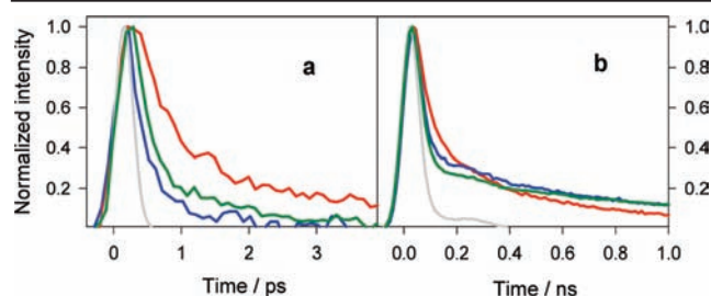
Figure 2. Fluorescence decays of DNA in phosphate buffer recorded at 305 nm (blue), 330 nm (green), and 420 nm (red) by FU (a) and TCSPC (b). The instrumental response functions are shown in gray.
