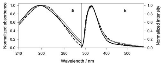
Figure 1. Normalized steady-state absorption (a) and fluorescence (b) spectra of DNA in pure water (gray) and in phosphate buffer (black). Excitation wavelength: 267 nm. The spectra of the stoichiometric mixture of monomers (58% of dAMP and TMP, 42% of dGMP and dCMP) in water are shown as dashes.
